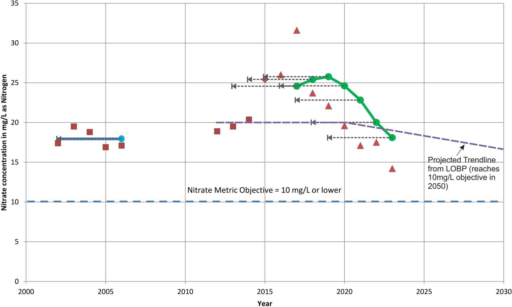
Figure 24 Nitrate Metric Los Osos Groundwater Basin 2023 Annual Report Cleath-Harris Geologists
