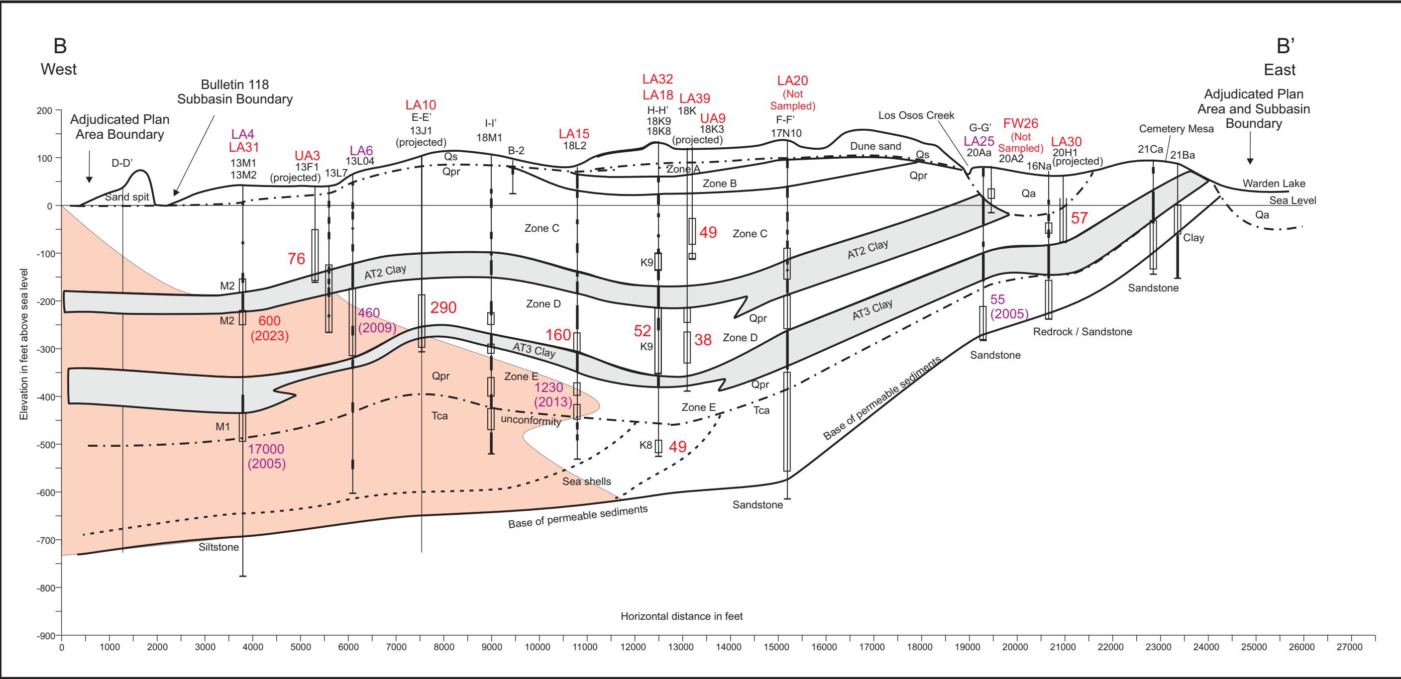
Figure 19 Seawater Intrusion Front Cross-Section B-B' Los Osos Groundwater Basin 2025 Annual Report Cleath-Harris Geologists
